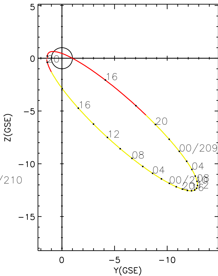
CLUSTER 2 orbit 2011 208 (07/27) 13:51 UT to 2011 210 (07/29) 20:11 UT
