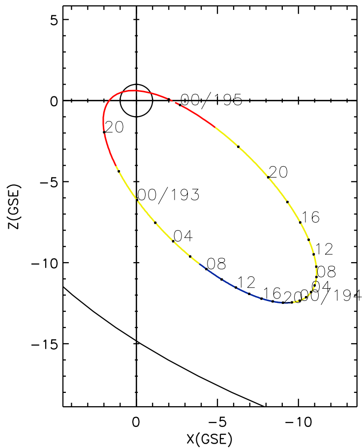
CLUSTER 2 orbit 2011 192 (07/11) 17:56 UT to 2011 195 (07/14) 00:06 UT
