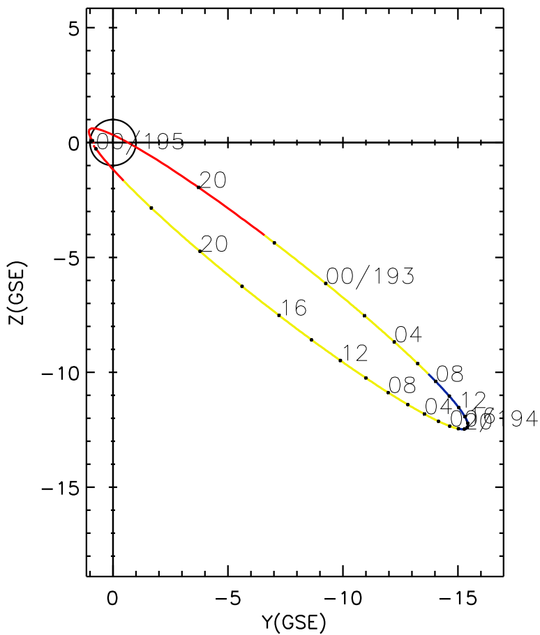
CLUSTER 2 orbit 2011 192 (07/11) 17:56 UT to 2011 195 (07/14) 00:06 UT
