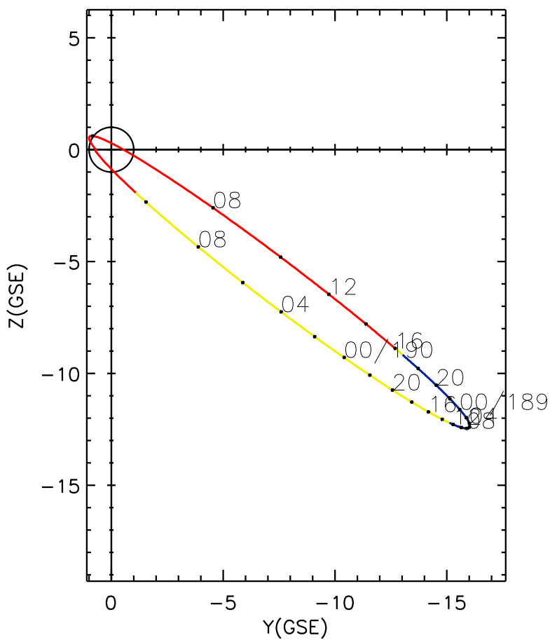
CLUSTER 2 orbit 2011 188 (07/07) 05:26 UT to 2011 190 (07/09) 11:41 UT
