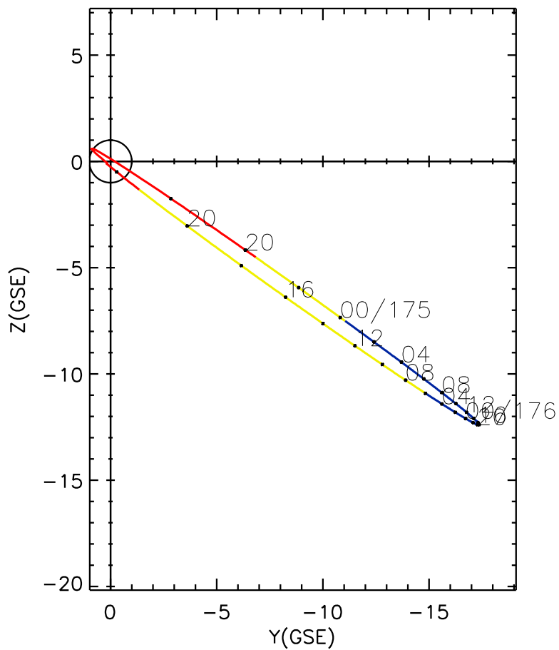
CLUSTER 2 orbit 2011 174 (06/23) 16:01 UT to 2011 176 (06/25) 22:16 UT
