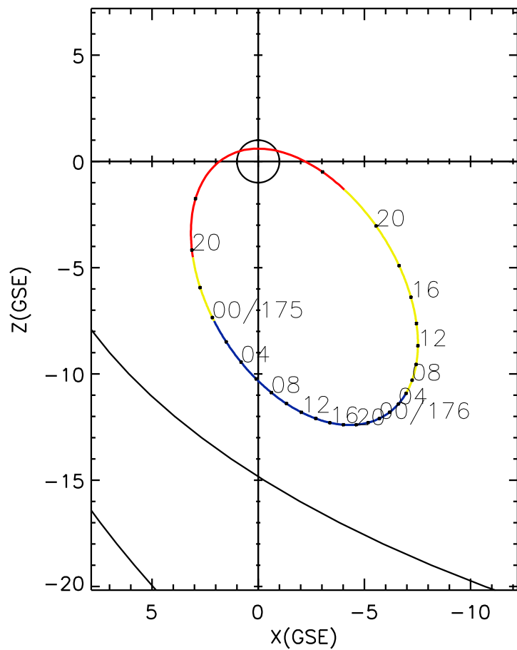
CLUSTER 2 orbit 2011 174 (06/23) 16:01 UT to 2011 176 (06/25) 22:16 UT
