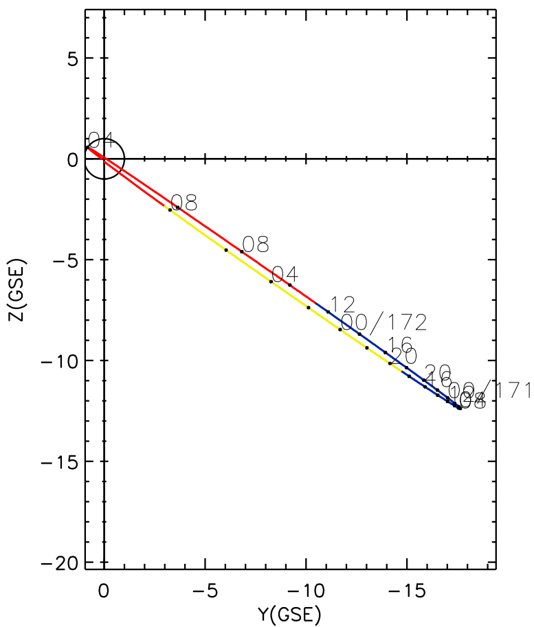
CLUSTER 2 orbit 2011 170 (06/19) 03:36 UT to 2011 172 (06/21) 09:46 UT
