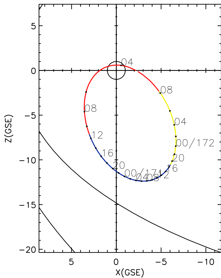
CLUSTER 2 orbit 2011 170 (06/19) 03:36 UT to 2011 172 (06/21) 09:46 UT
