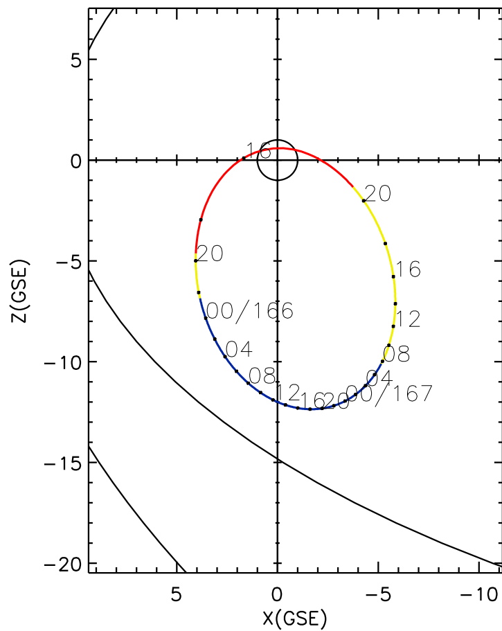
CLUSTER 2 orbit 2011 165 (06/14) 15:06 UT to 2011 167 (06/16) 21:21 UT
