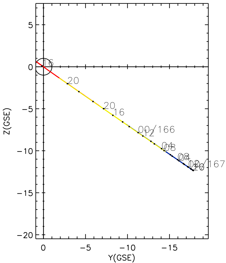
CLUSTER 2 orbit 2011 165 (06/14) 15:06 UT to 2011 167 (06/16) 21:21 UT
