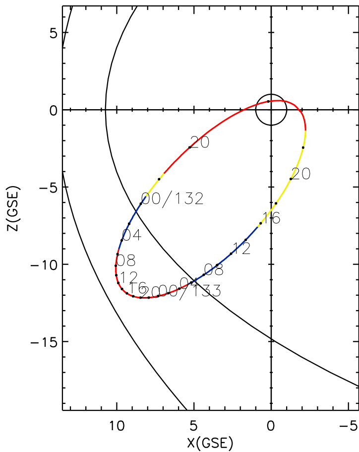
CLUSTER 2 orbit 2011 131 (05/11) 17:21 UT to 2011 133 (05/13) 23:41 UT
