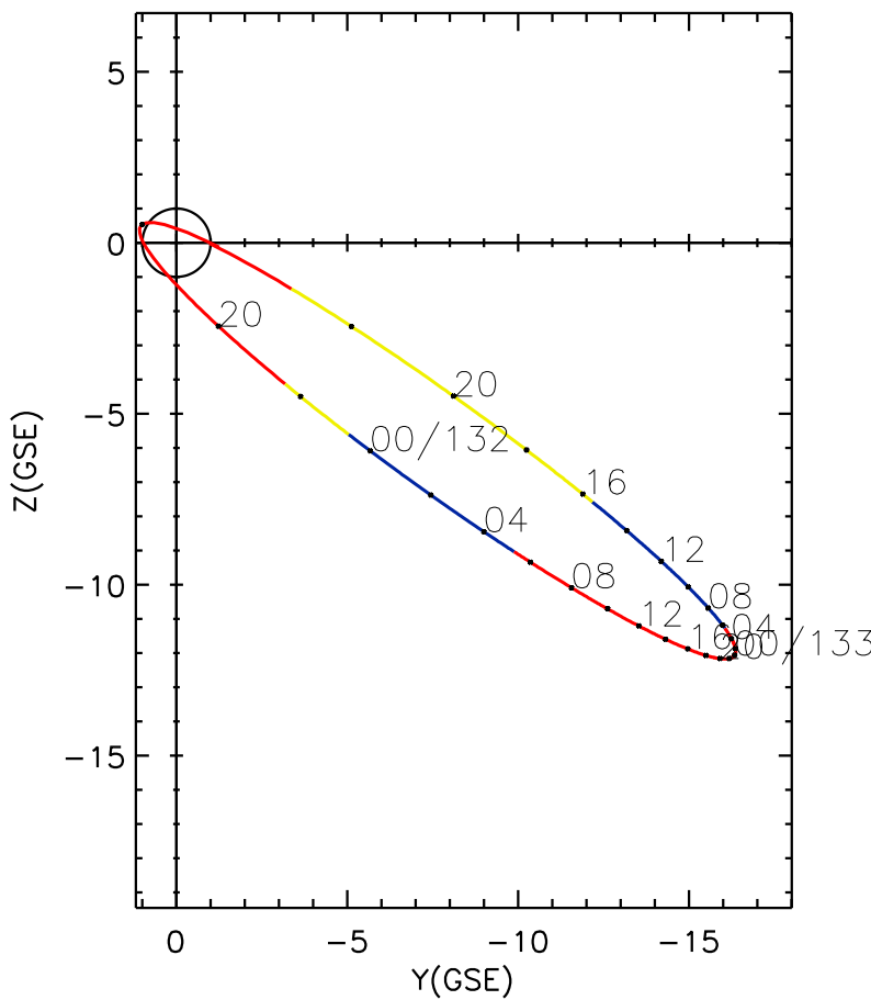
CLUSTER 2 orbit 2011 131 (05/11) 17:21 UT to 2011 133 (05/13) 23:41 UT
