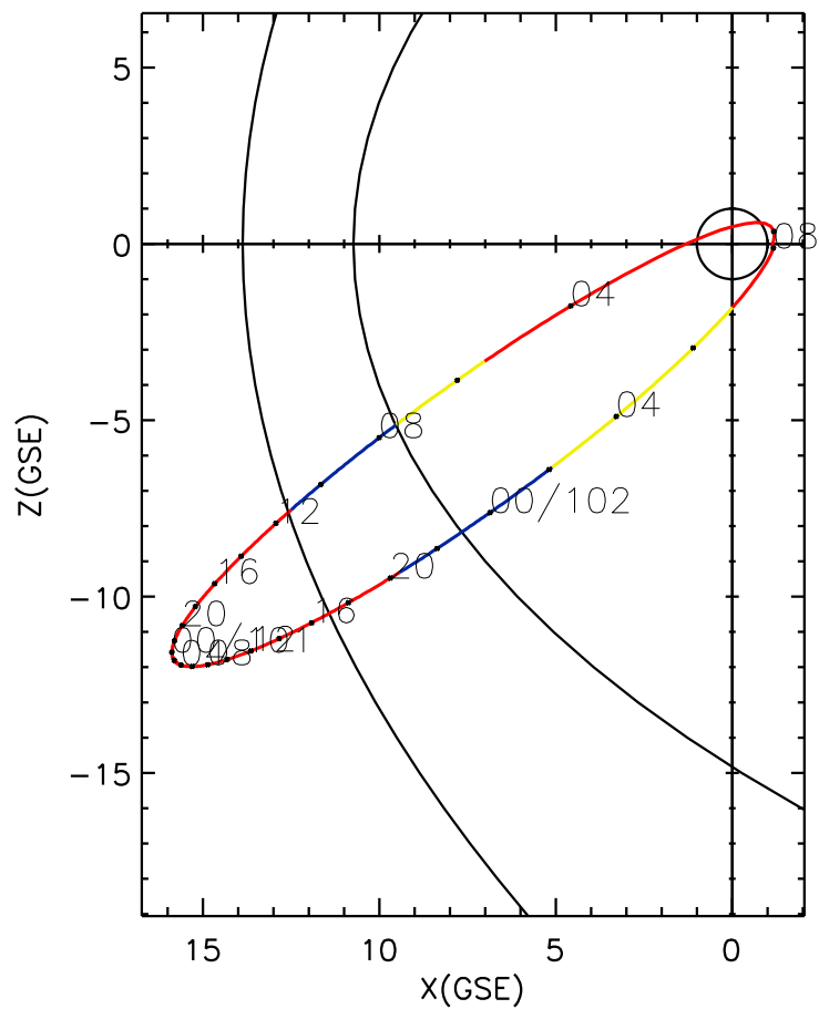
CLUSTER 2 orbit 2011 100 (04/10) 01:46 UT to 2011 102 (04/12) 08:01 UT
