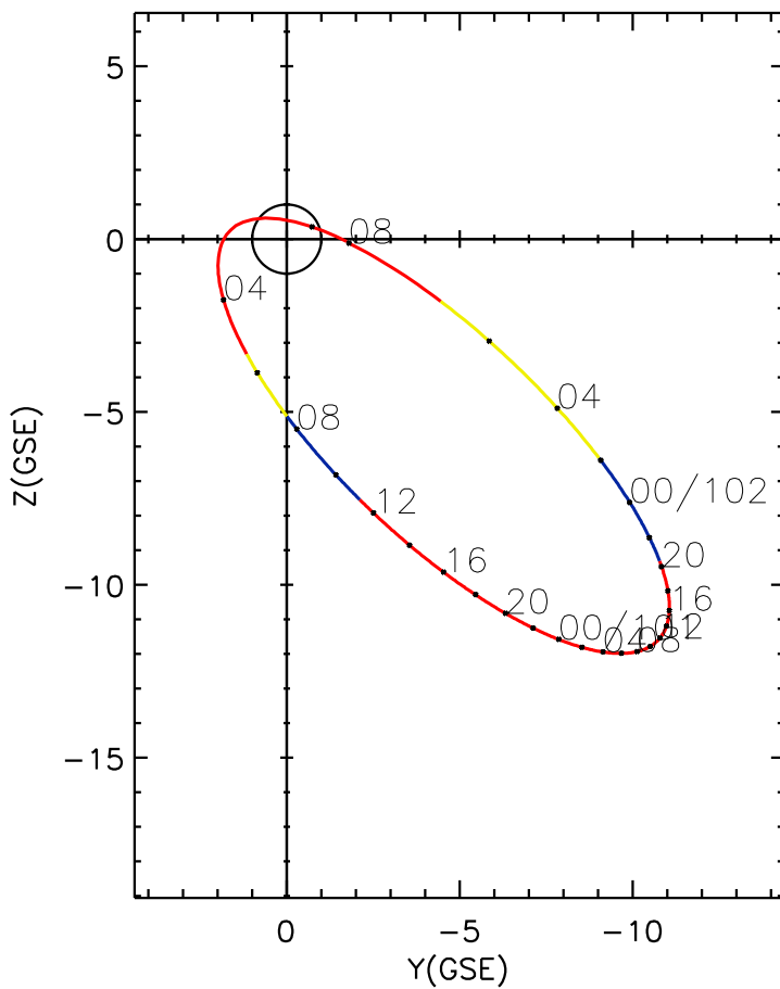
CLUSTER 2 orbit 2011 100 (04/10) 01:46 UT to 2011 102 (04/12) 08:01 UT
