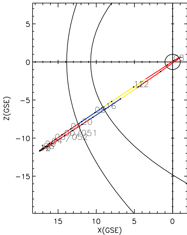
CLUSTER 2 orbit 2011 050 (02/19) 07:51 UT to 2011 052 (02/21) 14:11 UT
