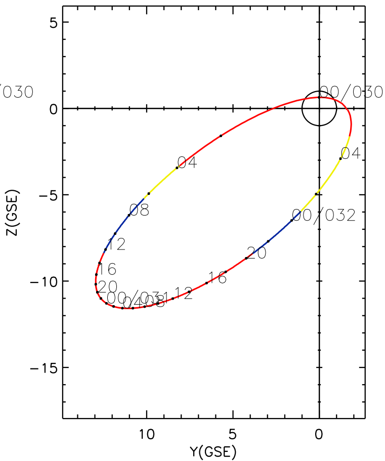
CLUSTER 2 orbit 2011 029 (01/29) 23:31 UT to 2011 032 (02/01) 05:46 UT
