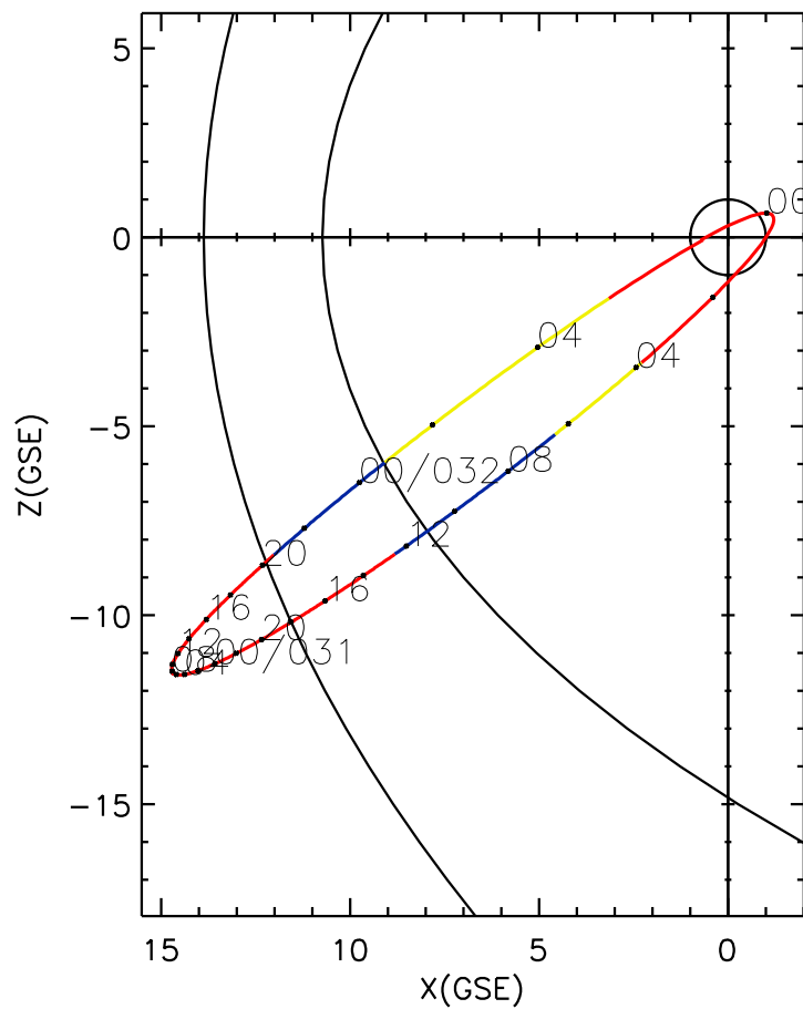
CLUSTER 2 orbit 2011 029 (01/29) 23:31 UT to 2011 032 (02/01) 05:46 UT
