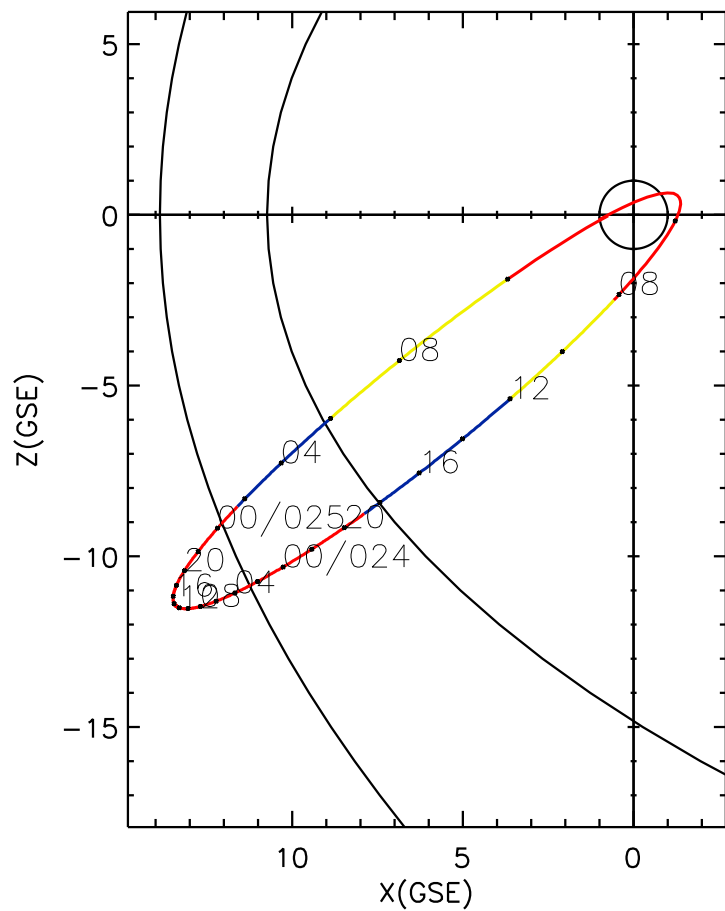
CLUSTER 2 orbit 2011 023 (01/23) 04:41 UT to 2011 025 (01/25) 11:01 UT
