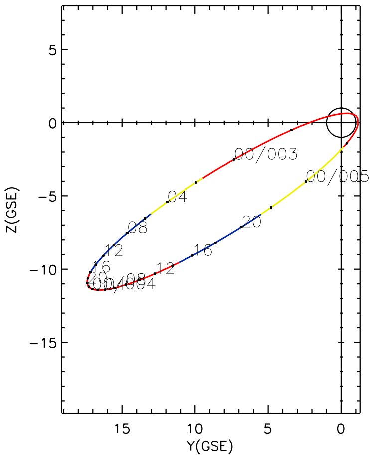
CLUSTER 2 orbit 2011 002 (01/02) 20:26 UT to 2011 005 (01/05) 02:41 UT
