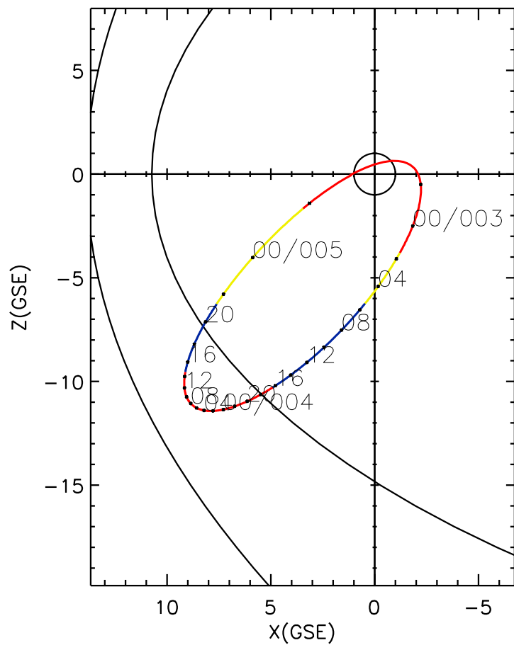
CLUSTER 2 orbit 2011 002 (01/02) 20:26 UT to 2011 005 (01/05) 02:41 UT
