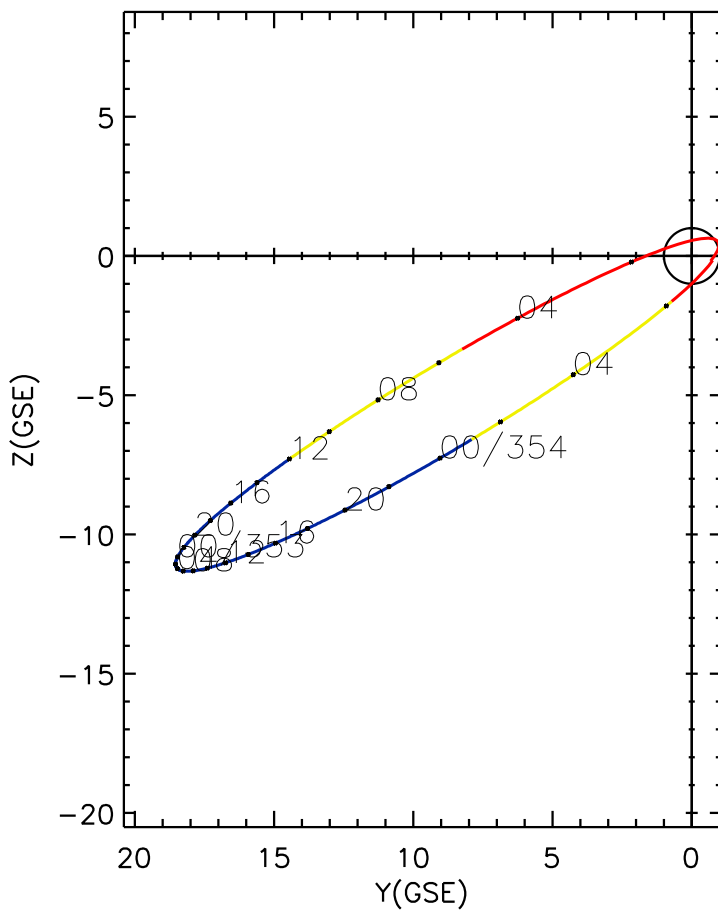
CLUSTER 2 orbit 2010 352 (12/18) 00:36 UT to 2010 354 (12/20) 06:51 UT
