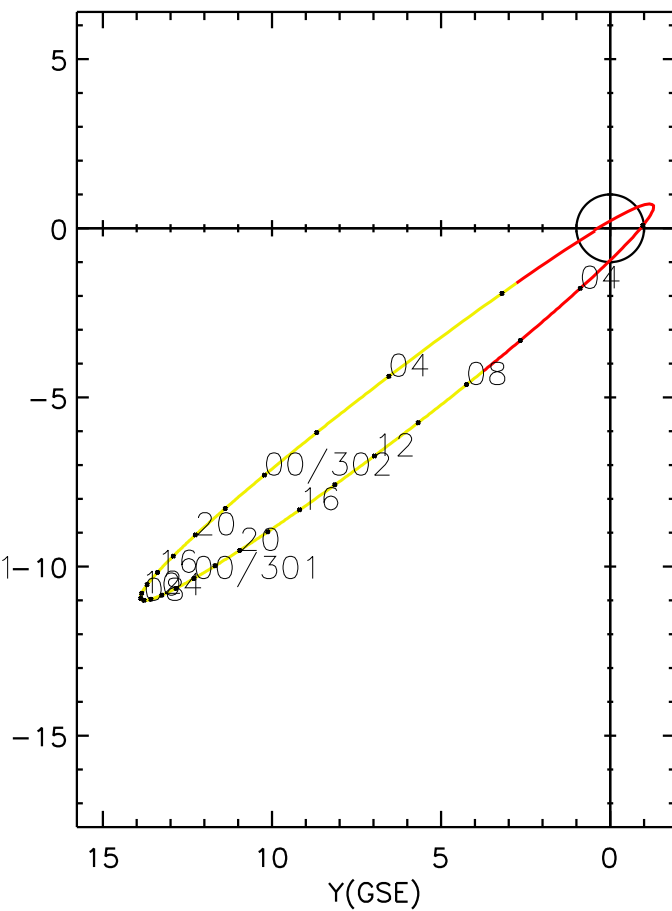
CLUSTER 2 orbit 2010 300 (10/27) 00:41 UT to 2010 302 (10/29) 06:56 UT
