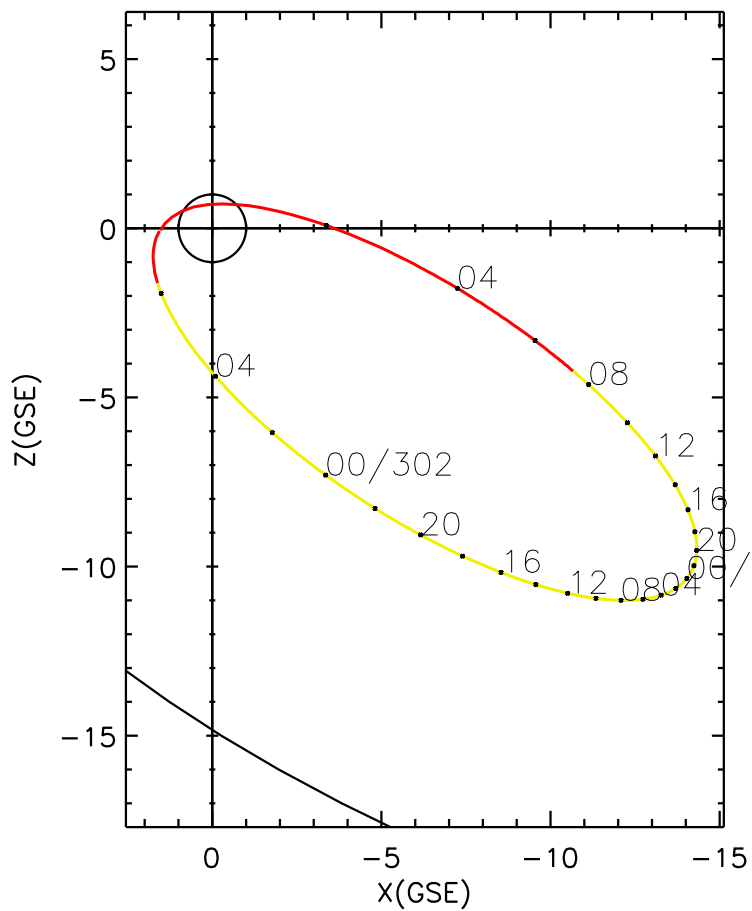
CLUSTER 2 orbit 2010 300 (10/27) 00:41 UT to 2010 302 (10/29) 06:56 UT
