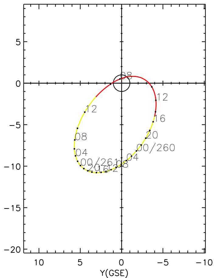
CLUSTER 2 orbit 2010 259 (09/16) 07:46 UT to 2010 261 (09/18) 14:01 UT
