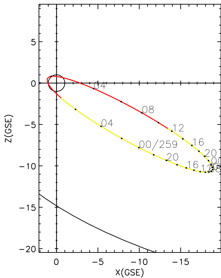
CLUSTER 2 orbit 2010 257 (09/14) 01:31 UT to 2010 259 (09/16) 07:46 UT
