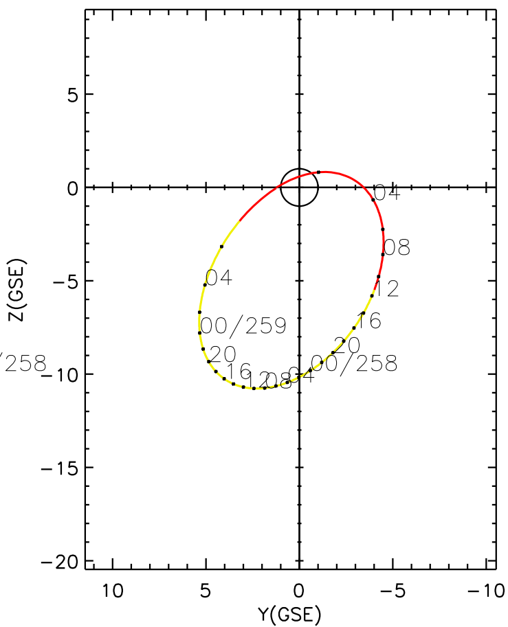
CLUSTER 2 orbit 2010 257 (09/14) 01:31 UT to 2010 259 (09/16) 07:46 UT
