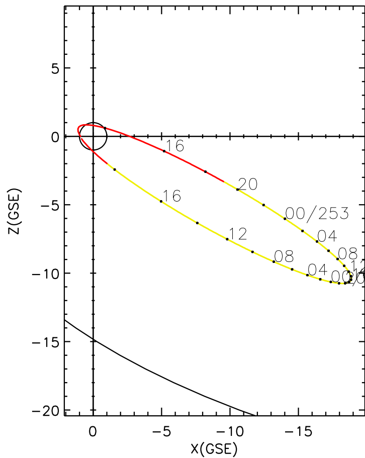
CLUSTER 2 orbit 2010 252 (09/09) 12:56 UT to 2010 254 (09/11) 19:11 UT
