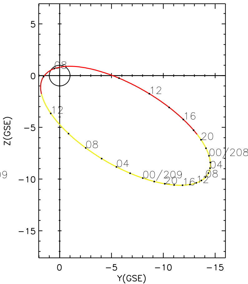
CLUSTER 2 orbit 2010 207 (07/26) 07:41 UT to 2010 209 (07/28) 14:01 UT
