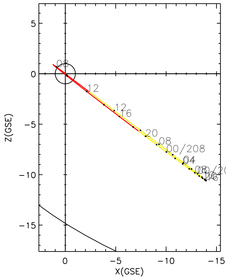
CLUSTER 2 orbit 2010 207 (07/26) 07:41 UT to 2010 209 (07/28) 14:01 UT
