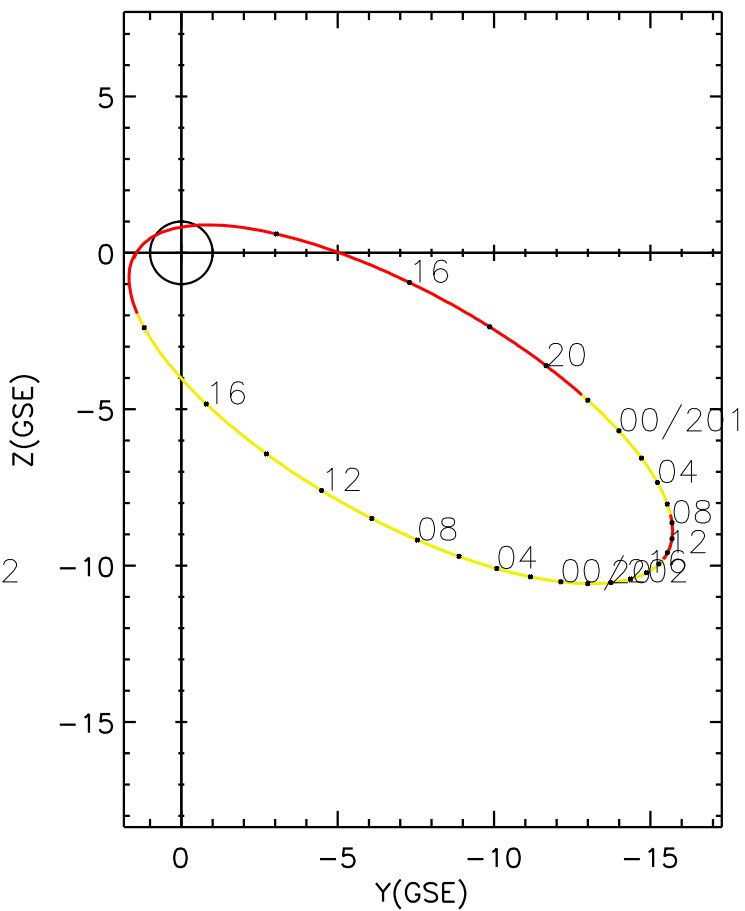
CLUSTER 2 orbit 2010 200 (07/19) 12:46 UT to 2010 202 (07/21) 19:06 UT
