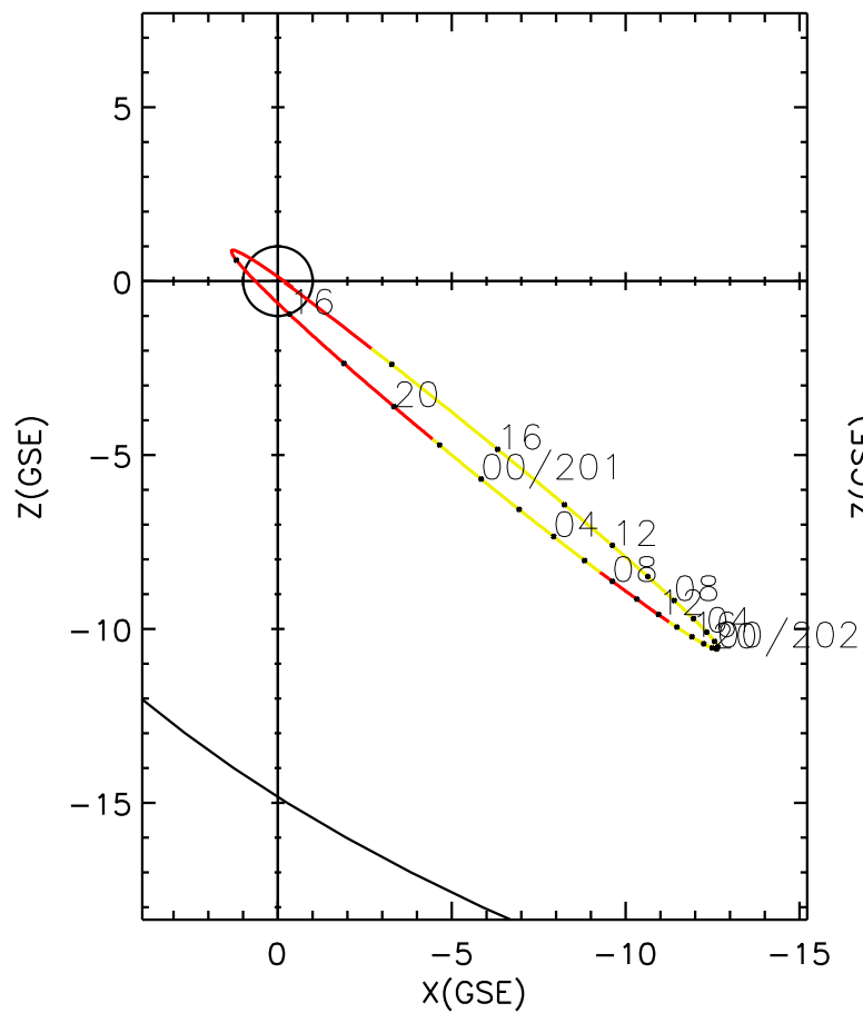
CLUSTER 2 orbit 2010 200 (07/19) 12:46 UT to 2010 202 (07/21) 19:06 UT
