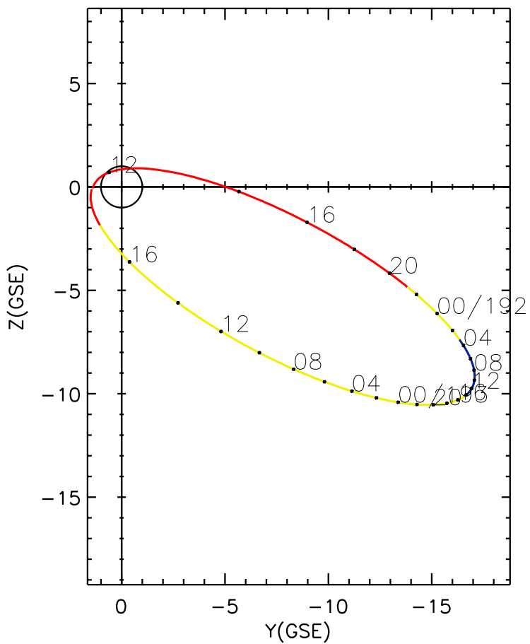
CLUSTER 2 orbit 2010 191 (07/10) 11:41 UT to 2010 193 (07/12) 17:56 UT
