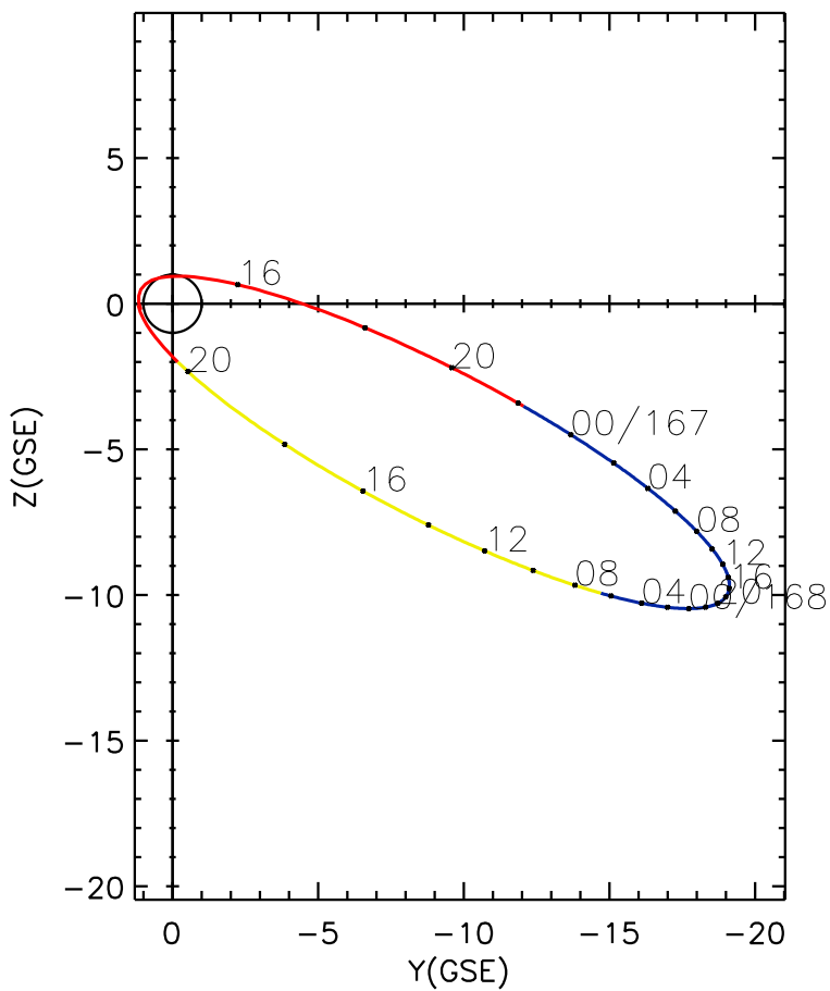
CLUSTER 2 orbit 2010 166 (06/15) 14:41 UT to 2010 168 (06/17) 21:01 UT
