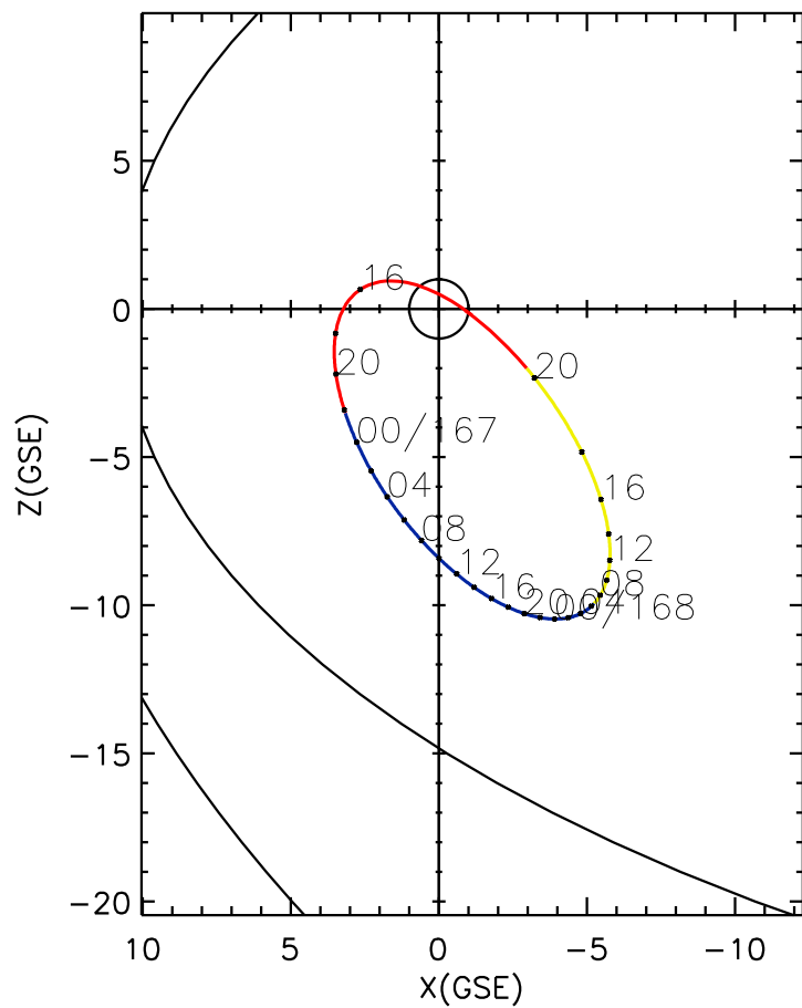
CLUSTER 2 orbit 2010 166 (06/15) 14:41 UT to 2010 168 (06/17) 21:01 UT
