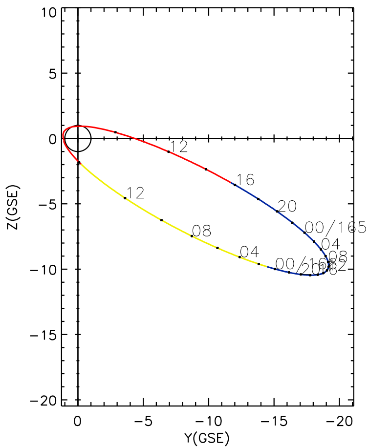
CLUSTER 2 orbit 2010 164 (06/13) 08:26 UT to 2010 166 (06/15) 14:41 UT
