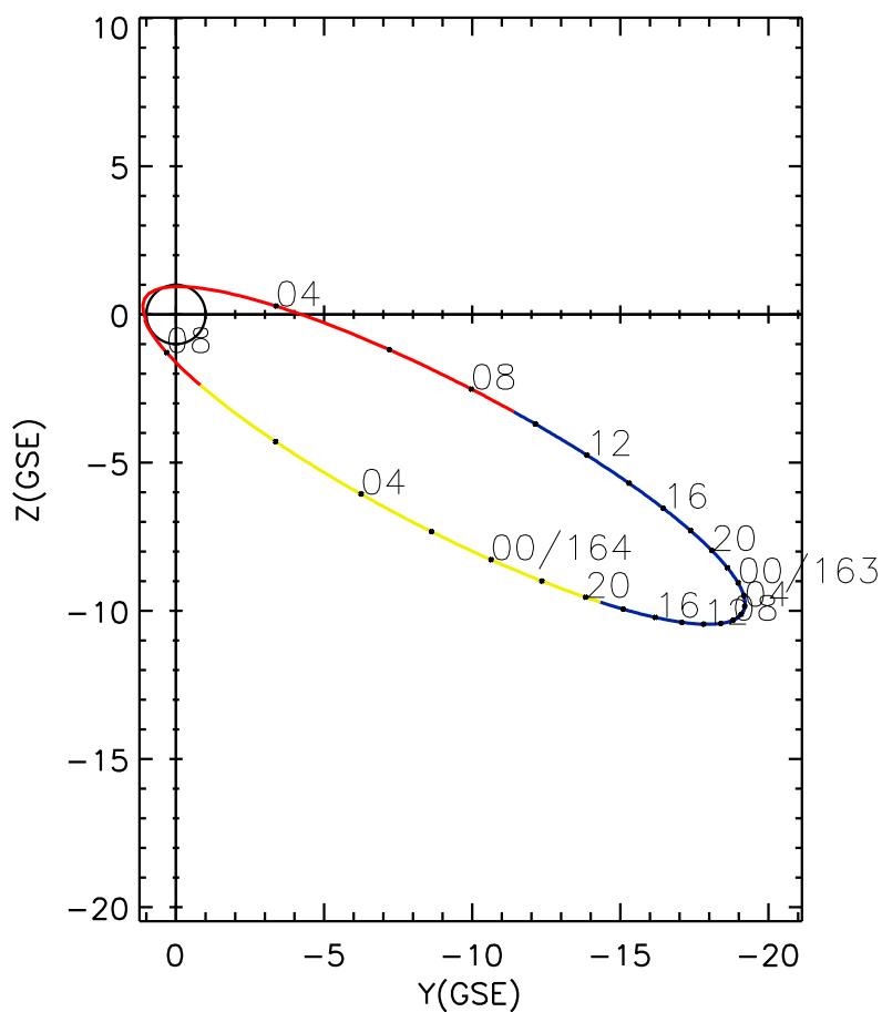
CLUSTER 2 orbit 2010 162 (06/11) 02:11 UT to 2010 164 (06/13) 08:26 UT
