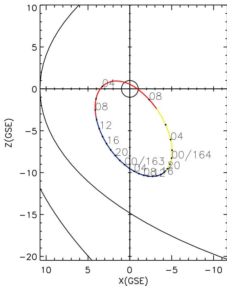
CLUSTER 2 orbit 2010 162 (06/11) 02:11 UT to 2010 164 (06/13) 08:26 UT
