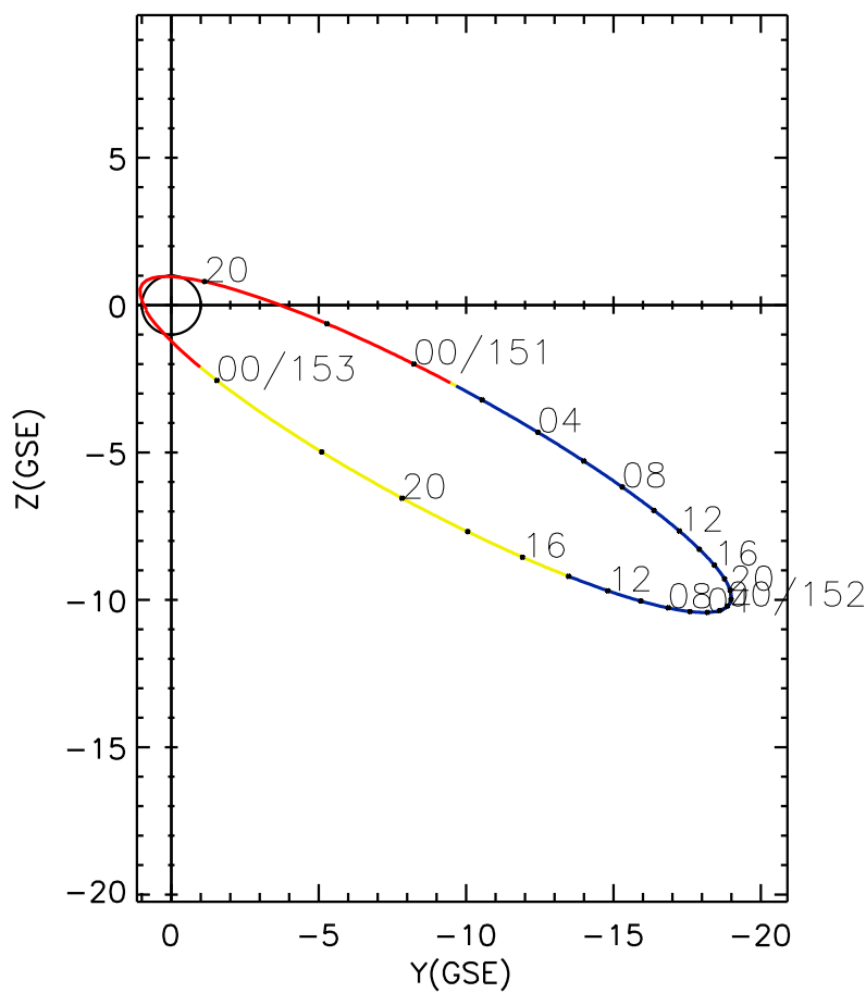
CLUSTER 2 orbit 2010 150 (05/30) 18:51 UT to 2010 153 (06/02) 01:06 UT
