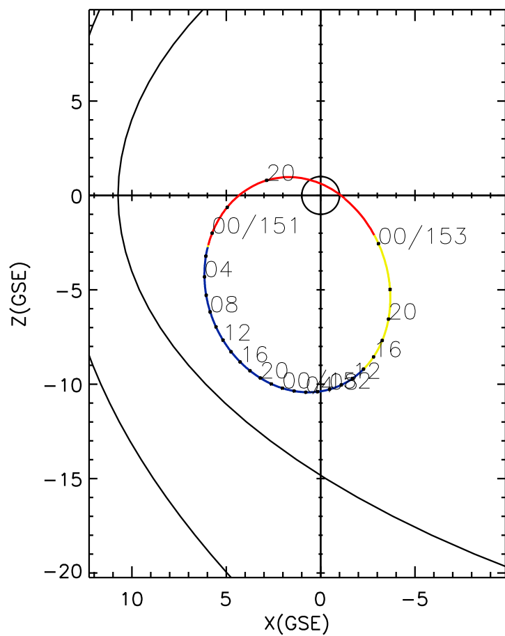
CLUSTER 2 orbit 2010 150 (05/30) 18:51 UT to 2010 153 (06/02) 01:06 UT
