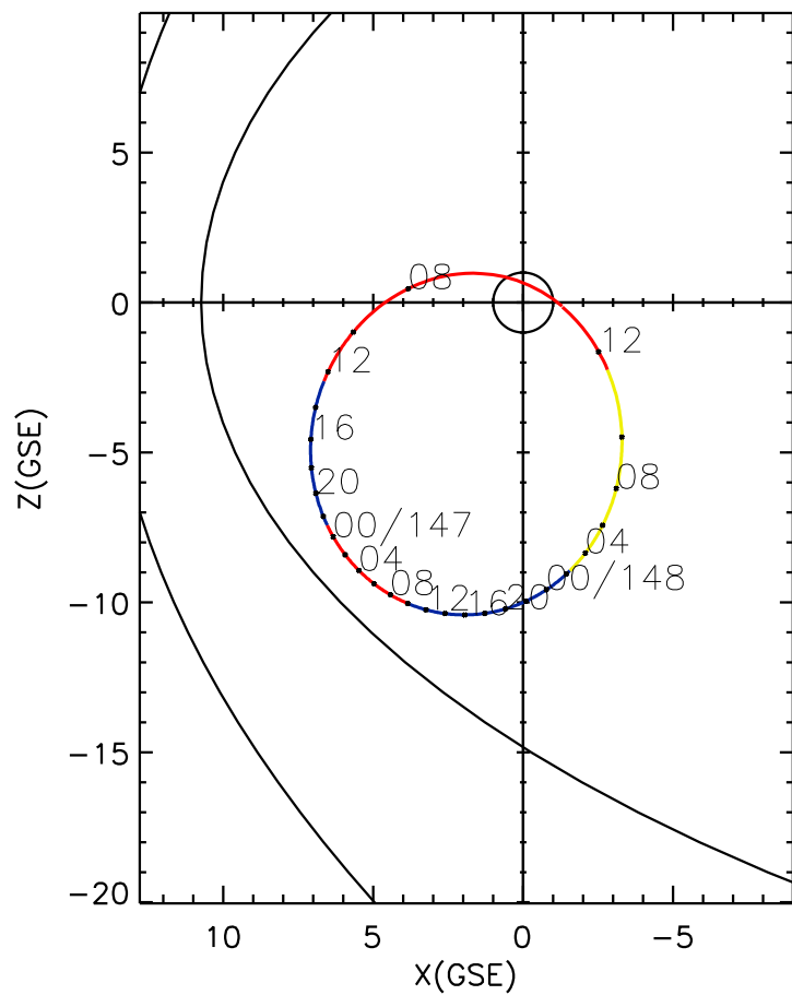
CLUSTER 2 orbit 2010 146 (05/26) 06:21 UT to 2010 148 (05/28) 12:36 UT
