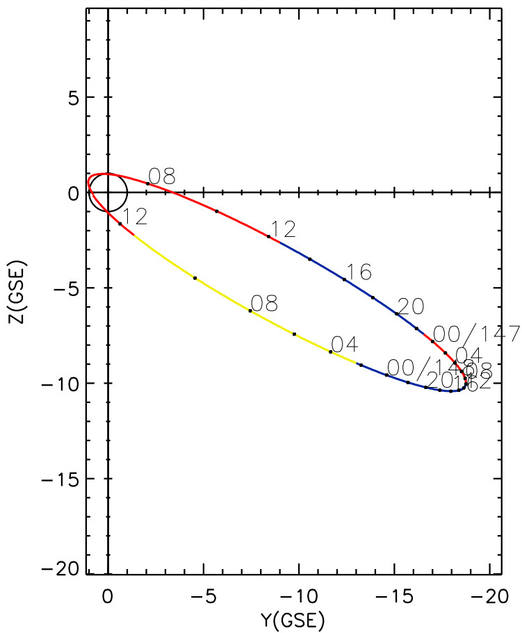
CLUSTER 2 orbit 2010 146 (05/26) 06:21 UT to 2010 148 (05/28) 12:36 UT
