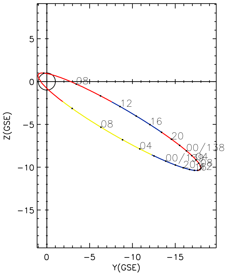
CLUSTER 2 orbit 2010 137 (05/17) 05:16 UT to 2010 139 (05/19) 11:31 UT
