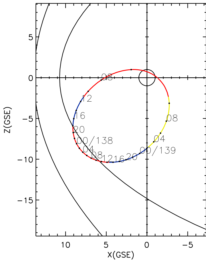
CLUSTER 2 orbit 2010 137 (05/17) 05:16 UT to 2010 139 (05/19) 11:31 UT
