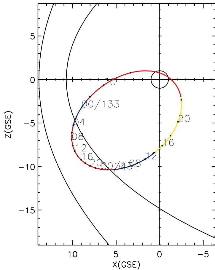
CLUSTER 2 orbit 2010 132 (05/12) 16:41 UT to 2010 134 (05/14) 23:01 UT
