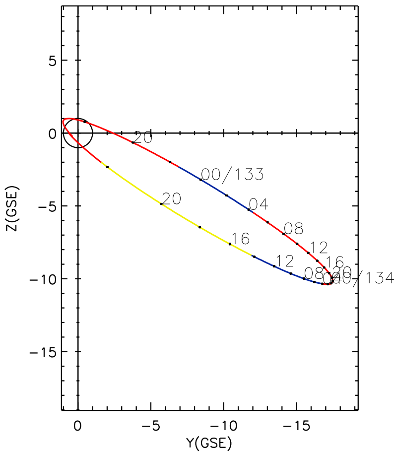
CLUSTER 2 orbit 2010 132 (05/12) 16:41 UT to 2010 134 (05/14) 23:01 UT
