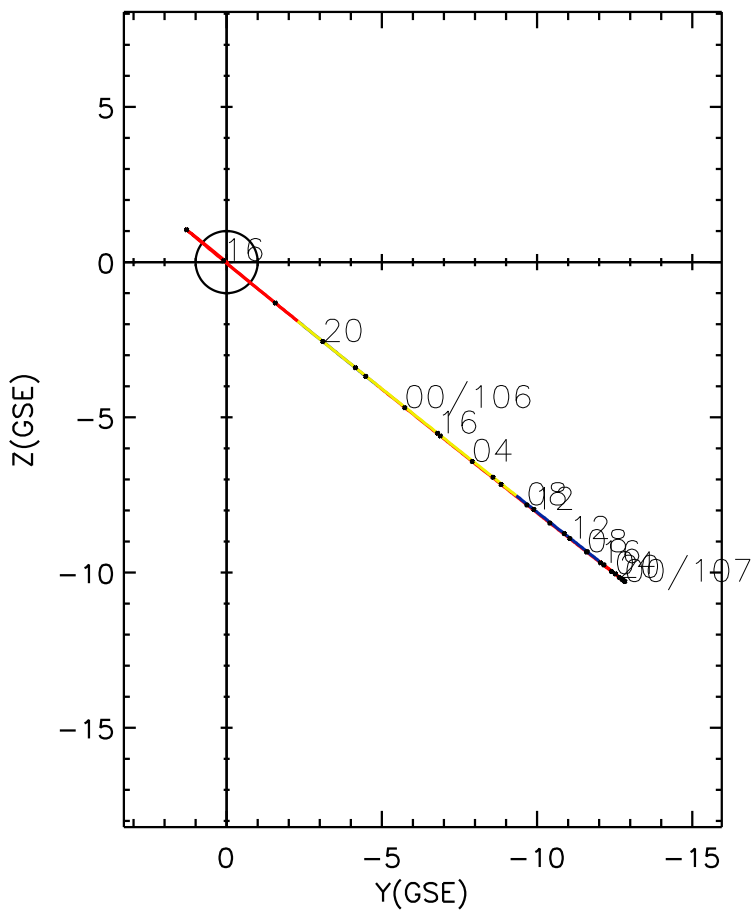
CLUSTER 2 orbit 2010 105 (04/15) 13:26 UT to 2010 107 (04/17) 19:41 UT
