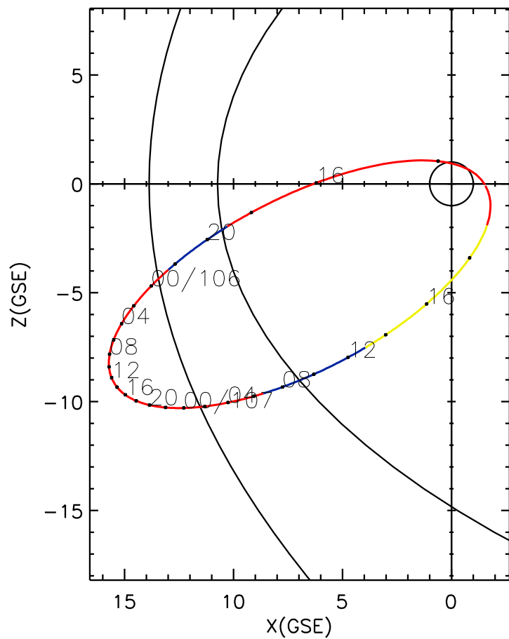
CLUSTER 2 orbit 2010 105 (04/15) 13:26 UT to 2010 107 (04/17) 19:41 UT
