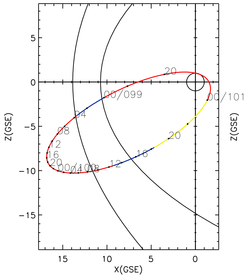
CLUSTER 2 orbit 2010 098 (04/08) 18:31 UT to 2010 101 (04/11) 00:51 UT
