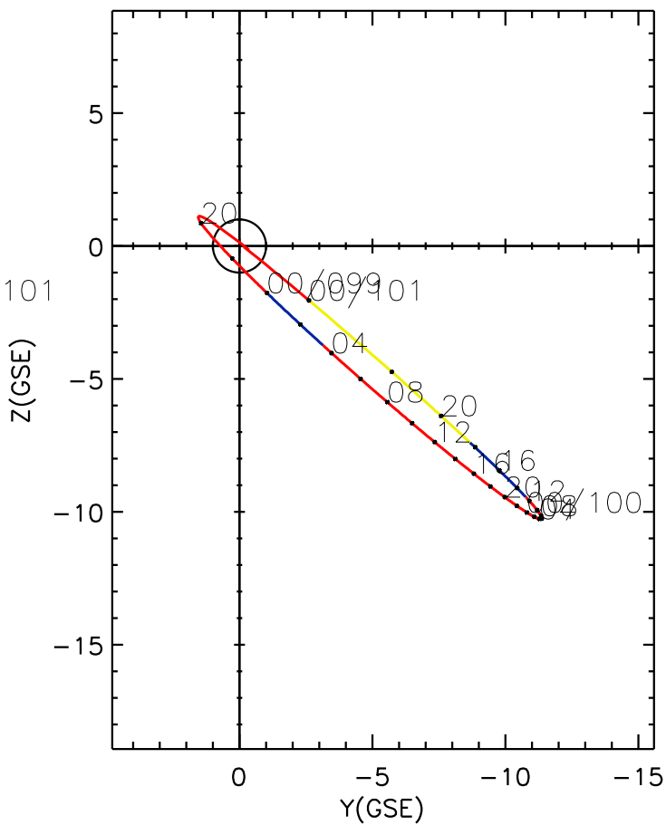
CLUSTER 2 orbit 2010 098 (04/08) 18:31 UT to 2010 101 (04/11) 00:51 UT
