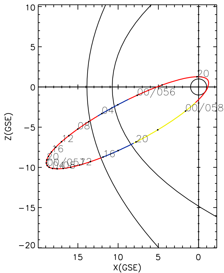
CLUSTER 2 orbit 2010 055 (02/24) 19:01 UT to 2010 058 (02/27) 01:21 UT
