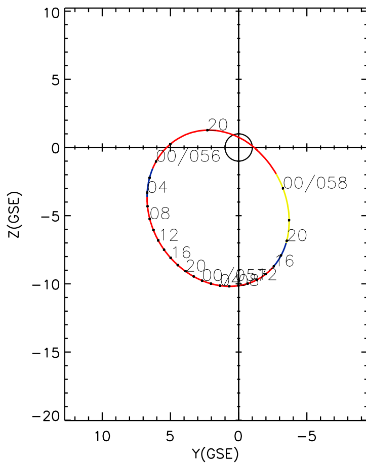
CLUSTER 2 orbit 2010 055 (02/24) 19:01 UT to 2010 058 (02/27) 01:21 UT
