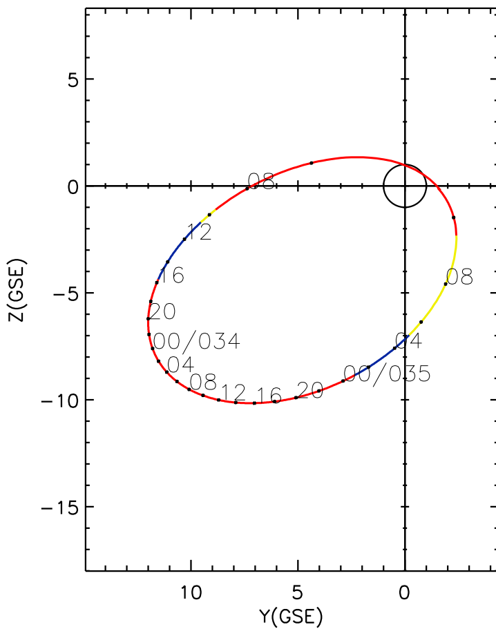
CLUSTER 2 orbit 2010 033 (02/02) 04:11 UT to 2010 035 (02/04) 10:31 UT
