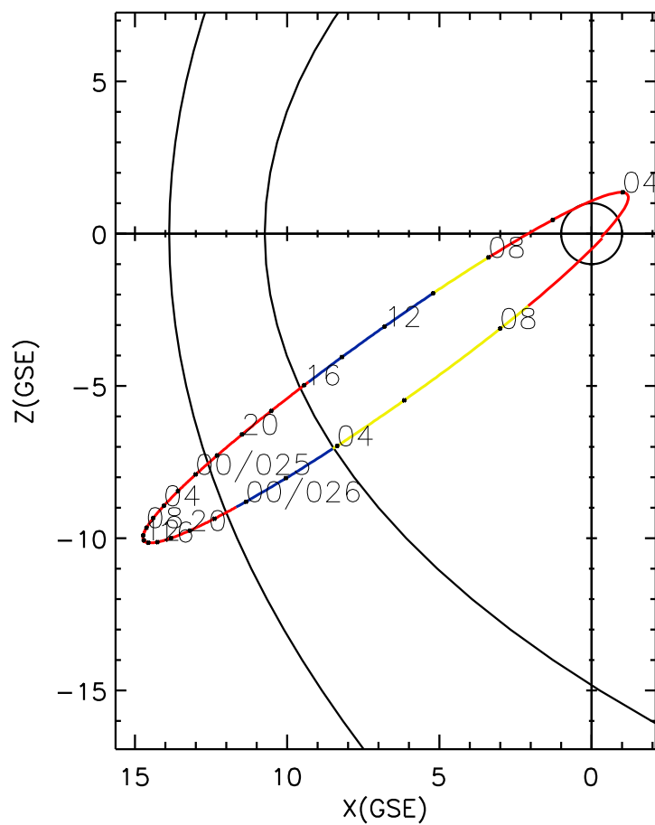
CLUSTER 2 orbit 2010 024 (01/24) 03:06 UT to 2010 026 (01/26) 09:21 UT
