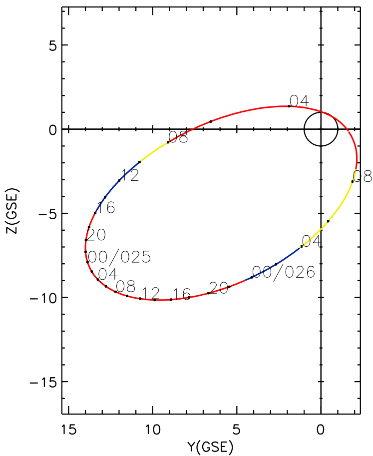
CLUSTER 2 orbit 2010 024 (01/24) 03:06 UT to 2010 026 (01/26) 09:21 UT
