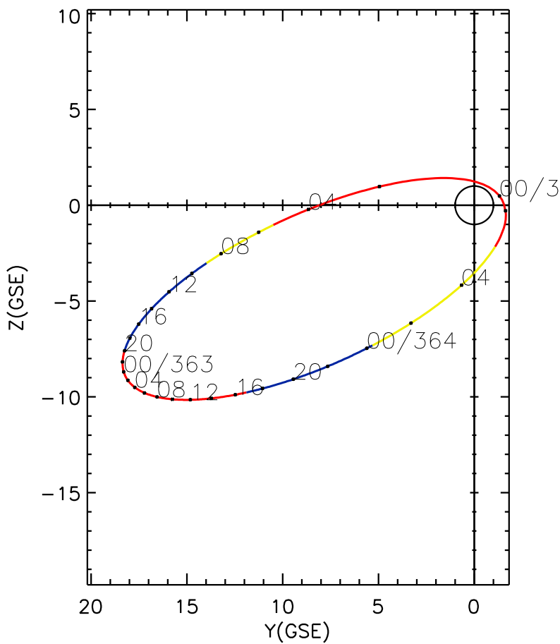
CLUSTER 2 orbit 2009 361 (12/27) 23:46 UT to 2009 364 (12/30) 06:01 UT
