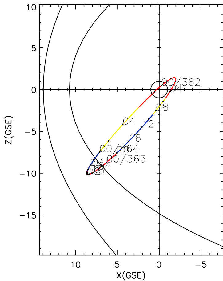
CLUSTER 2 orbit 2009 361 (12/27) 23:46 UT to 2009 364 (12/30) 06:01 UT
