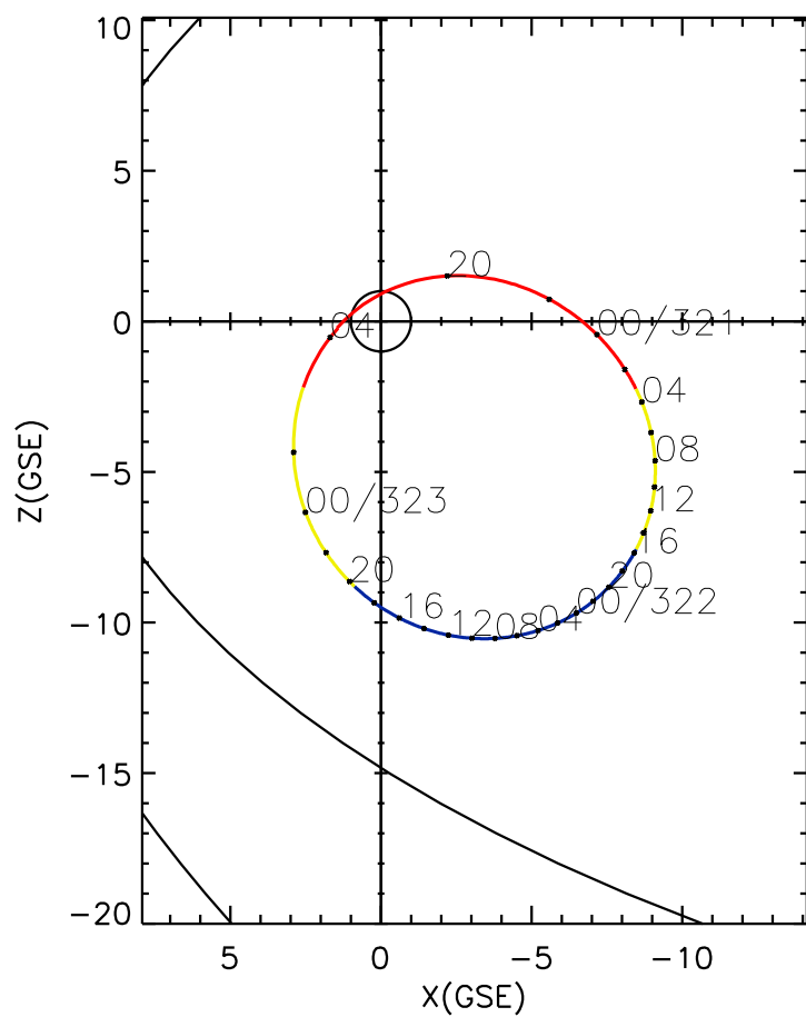
CLUSTER 2 orbit 2009 320 (11/16) 19:01 UT to 2009 323 (11/19) 04:06 UT
