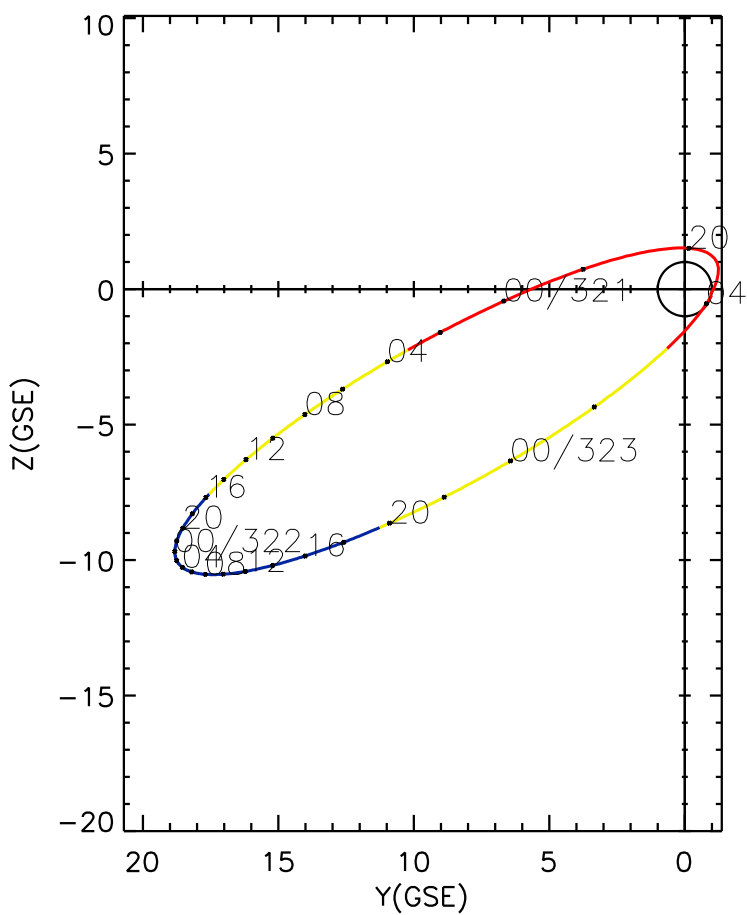
CLUSTER 2 orbit 2009 320 (11/16) 19:01 UT to 2009 323 (11/19) 04:06 UT
