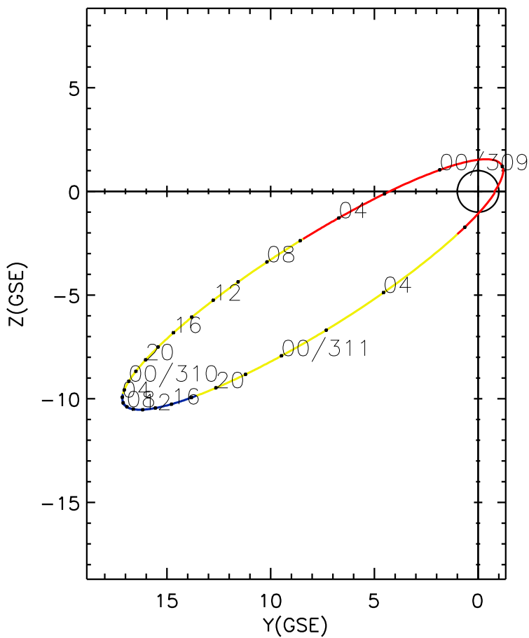
CLUSTER 2 orbit 2009 308 (11/04) 21:31 UT to 2009 311 (11/07) 06:36 UT
