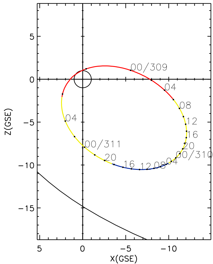
CLUSTER 2 orbit 2009 308 (11/04) 21:31 UT to 2009 311 (11/07) 06:36 UT
