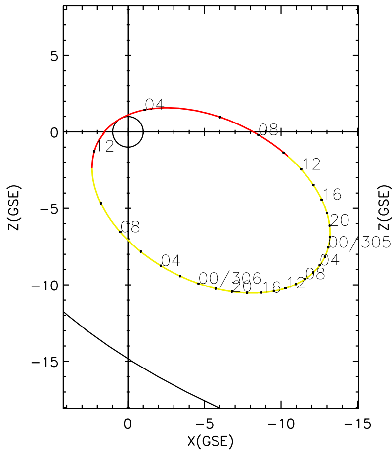
CLUSTER 2 orbit 2009 304 (10/31) 03:16 UT to 2009 306 (11/02) 12:26 UT
