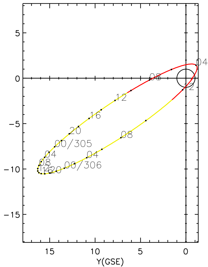
CLUSTER 2 orbit 2009 304 (10/31) 03:16 UT to 2009 306 (11/02) 12:26 UT
