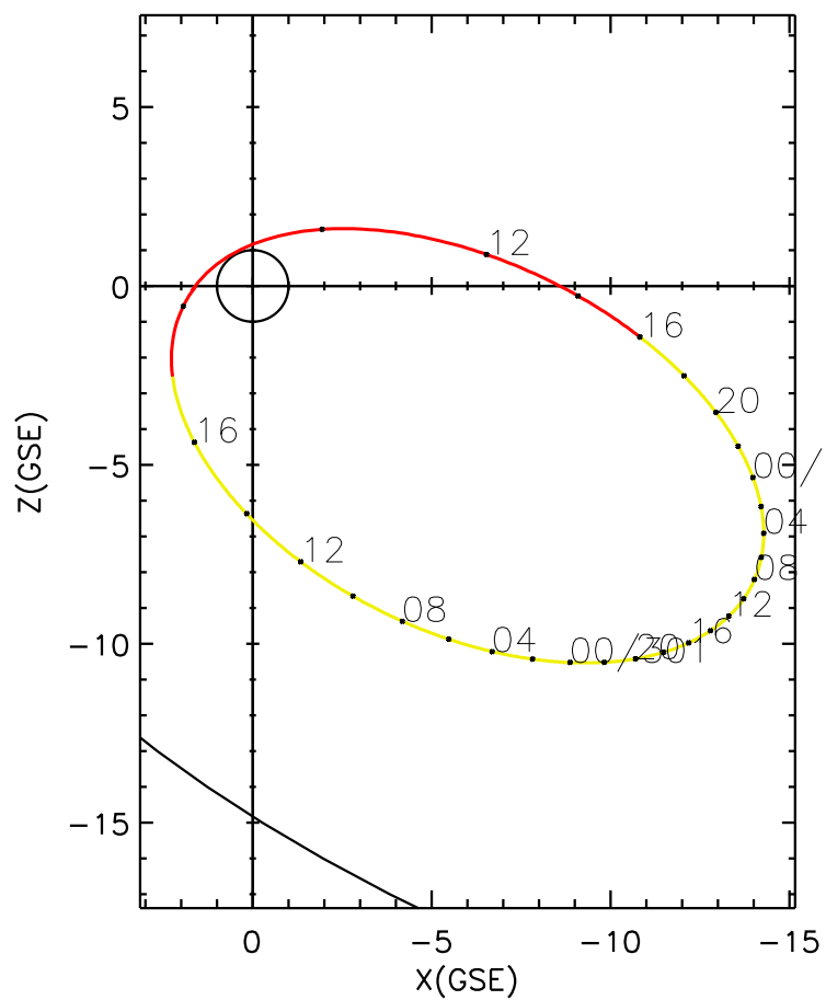
CLUSTER 2 orbit 2009 299 (10/26) 09:01 UT to 2009 301 (10/28) 18:11 UT
