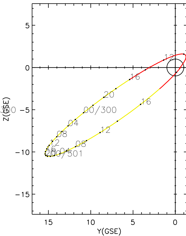
CLUSTER 2 orbit 2009 299 (10/26) 09:01 UT to 2009 301 (10/28) 18:11 UT
