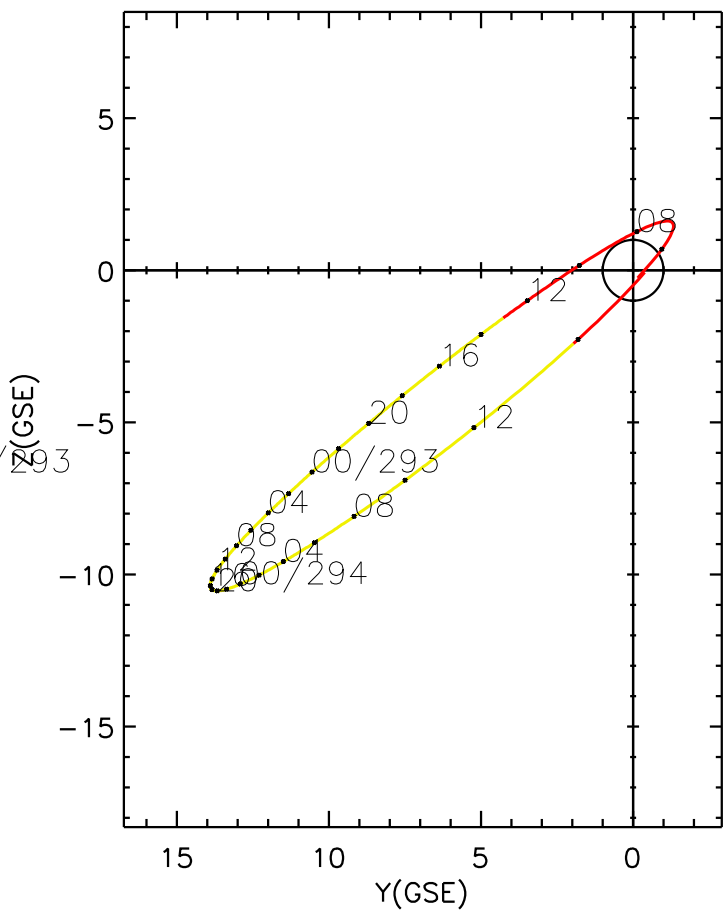
CLUSTER 2 orbit 2009 292 (10/19) 05:41 UT to 2009 294 (10/21) 14:51 UT
