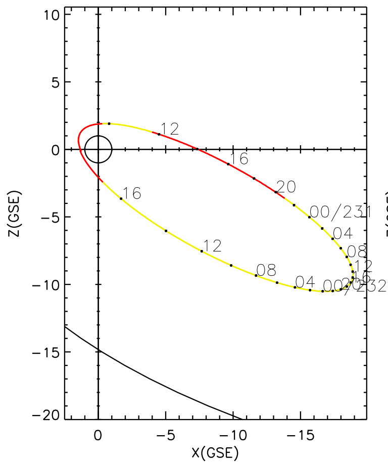
CLUSTER 2 orbit 2009 230 (08/18) 08:26 UT to 2009 232 (08/20) 17:36 UT
