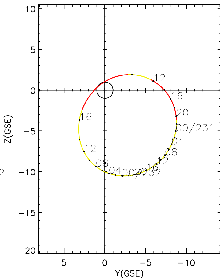
CLUSTER 2 orbit 2009 230 (08/18) 08:26 UT to 2009 232 (08/20) 17:36 UT
