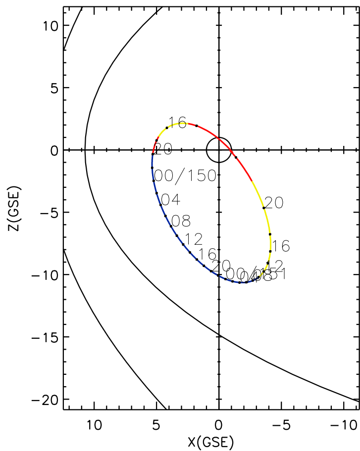
CLUSTER 2 orbit 2009 149 (05/29) 13:01 UT to 2009 151 (05/31) 22:10 UT
