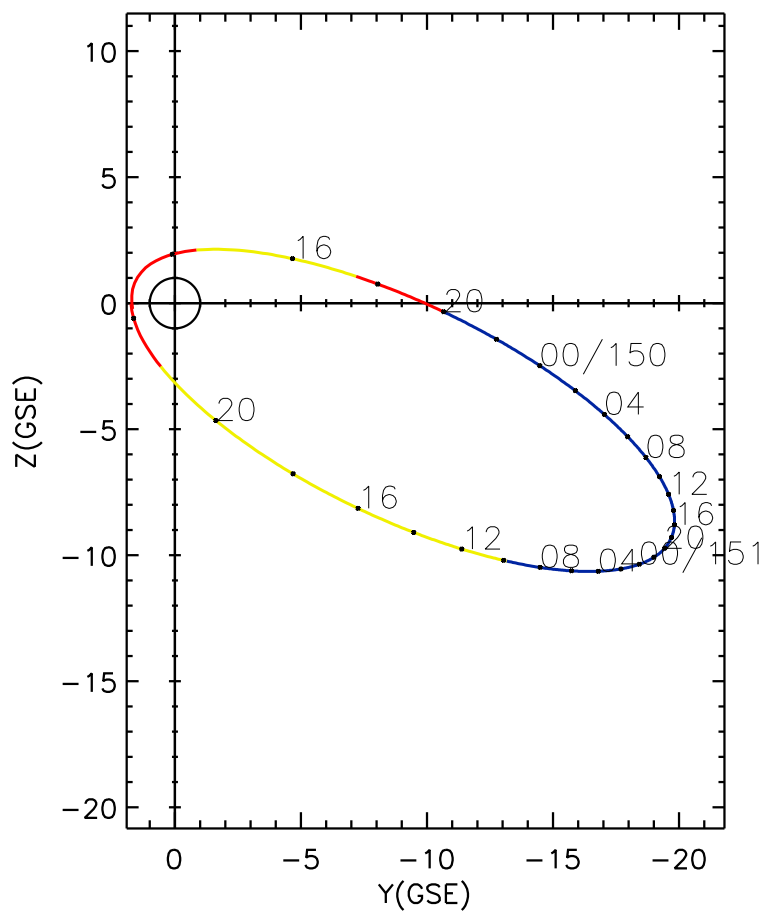
CLUSTER 2 orbit 2009 149 (05/29) 13:01 UT to 2009 151 (05/31) 22:10 UT
