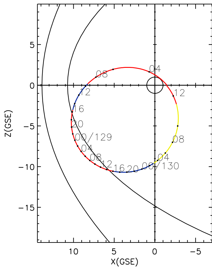
CLUSTER 2 orbit 2009 128 (05/08) 03:21 UT to 2009 130 (05/10) 12:26 UT
