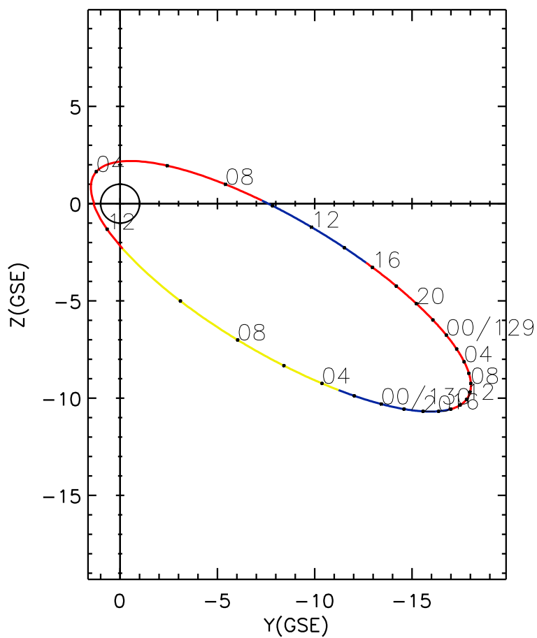
CLUSTER 2 orbit 2009 128 (05/08) 03:21 UT to 2009 130 (05/10) 12:26 UT
