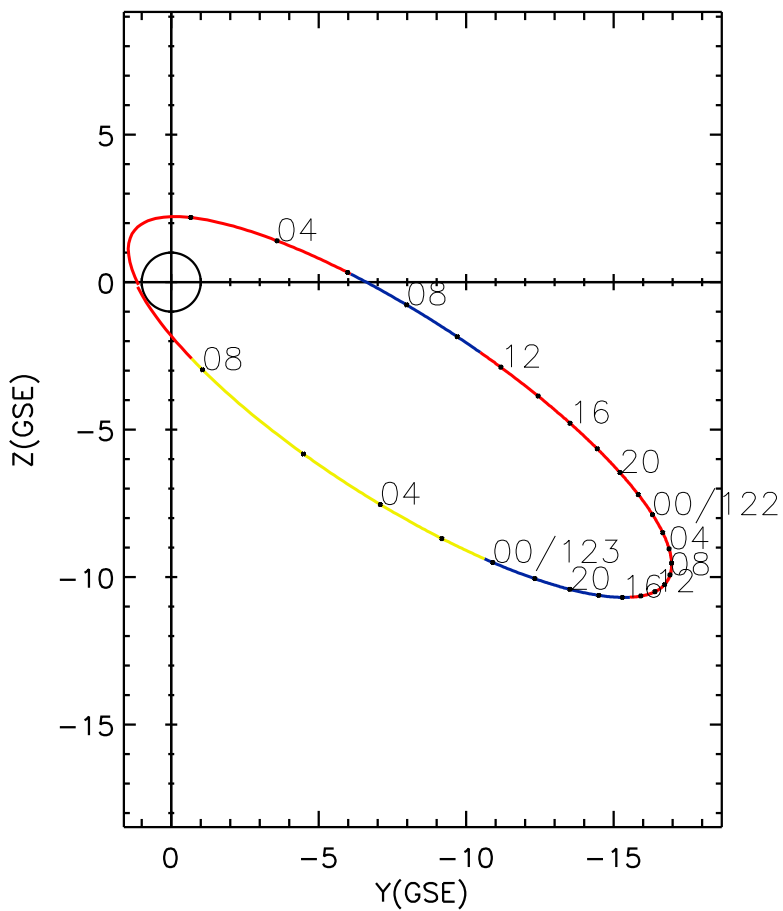
CLUSTER 2 orbit 2009 121 (05/01) 00:01 UT to 2009 123 (05/03) 09:06 UT
