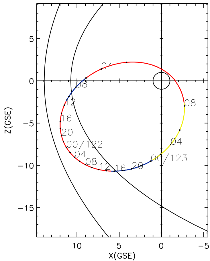
CLUSTER 2 orbit 2009 121 (05/01) 00:01 UT to 2009 123 (05/03) 09:06 UT
