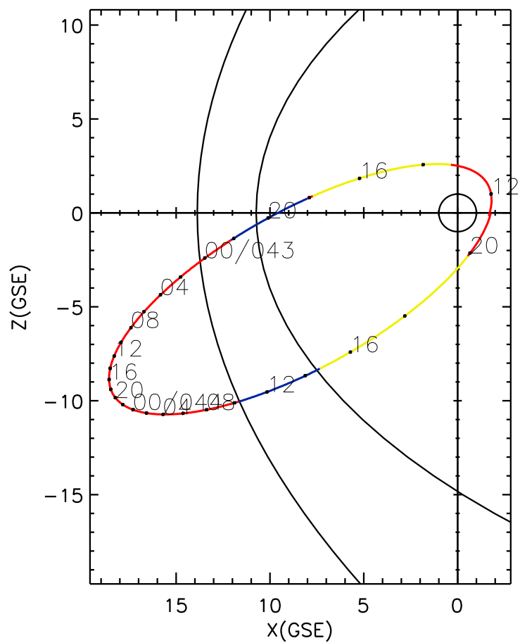
CLUSTER 2 orbit 2009 042 (02/11) 11:36 UT to 2009 044 (02/13) 20:46 UT
