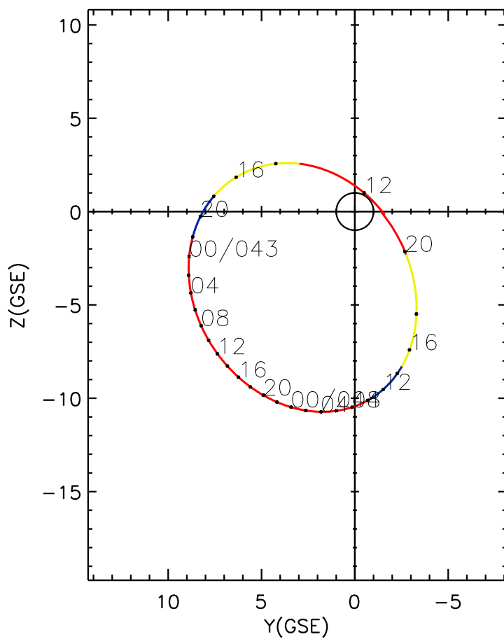
CLUSTER 2 orbit 2009 042 (02/11) 11:36 UT to 2009 044 (02/13) 20:46 UT
