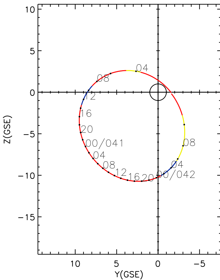
CLUSTER 2 orbit 2009 040 (02/09) 02:31 UT to 2009 042 (02/11) 11:36 UT
