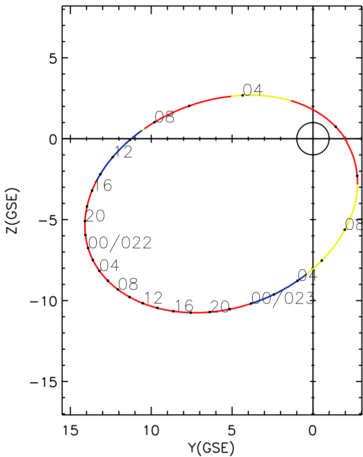
CLUSTER 2 orbit 2009 021 (01/21) 01:41 UT to 2009 023 (01/23) 10:46 UT
