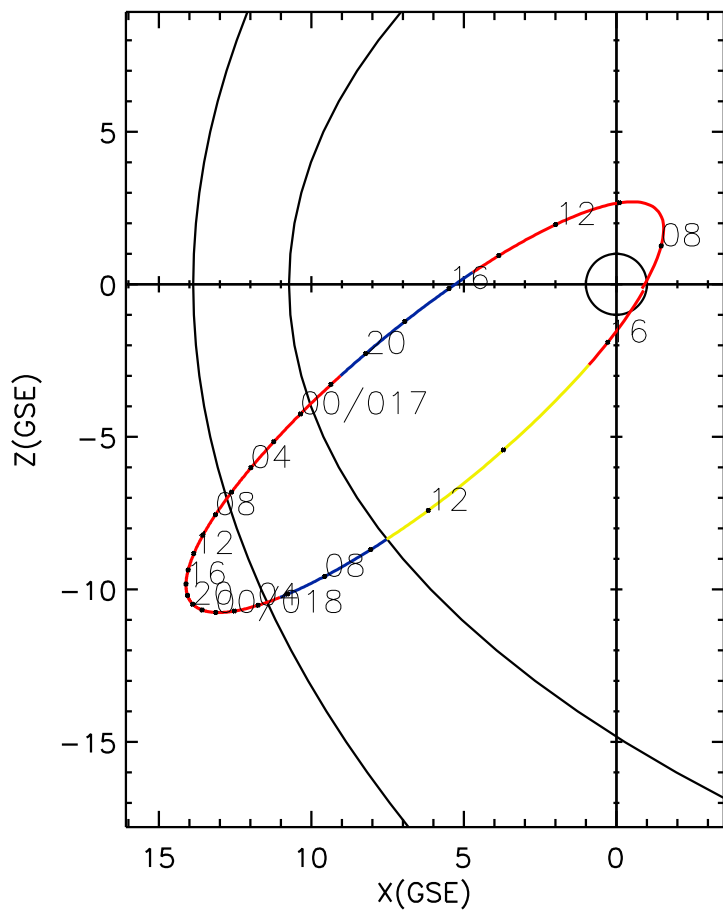
CLUSTER 2 orbit 2009 016 (01/16) 07:31 UT to 2009 018 (01/18) 16:36 UT
