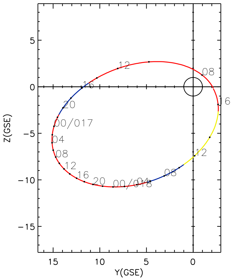
CLUSTER 2 orbit 2009 016 (01/16) 07:31 UT to 2009 018 (01/18) 16:36 UT
