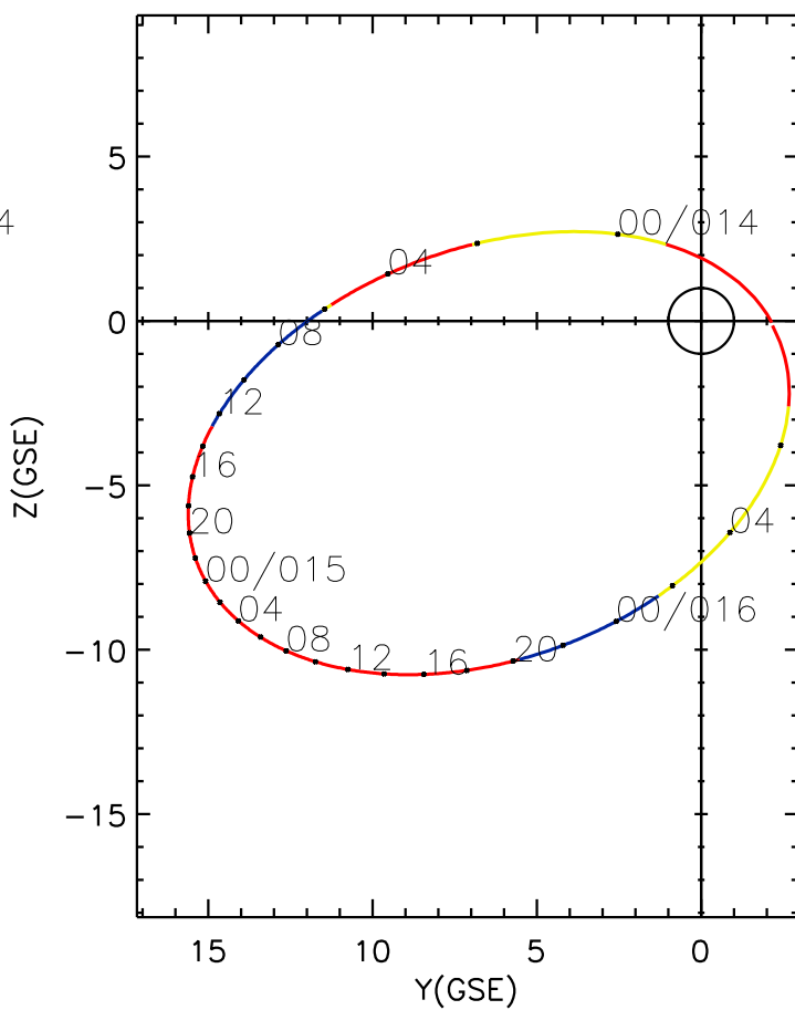
CLUSTER 2 orbit 2009 013 (01/13) 22:26 UT to 2009 016 (01/16) 07:31 UT
