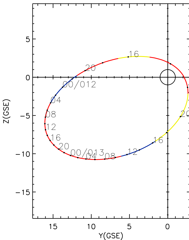
CLUSTER 2 orbit 2009 011 (01/11) 13:16 UT to 2009 013 (01/13) 22:26 UT
