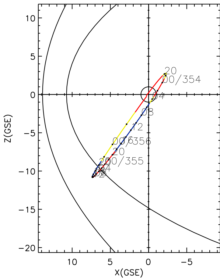
CLUSTER 2 orbit 2008 353 (12/18) 18:25 UT to 2008 356 (12/21) 03:31 UT
