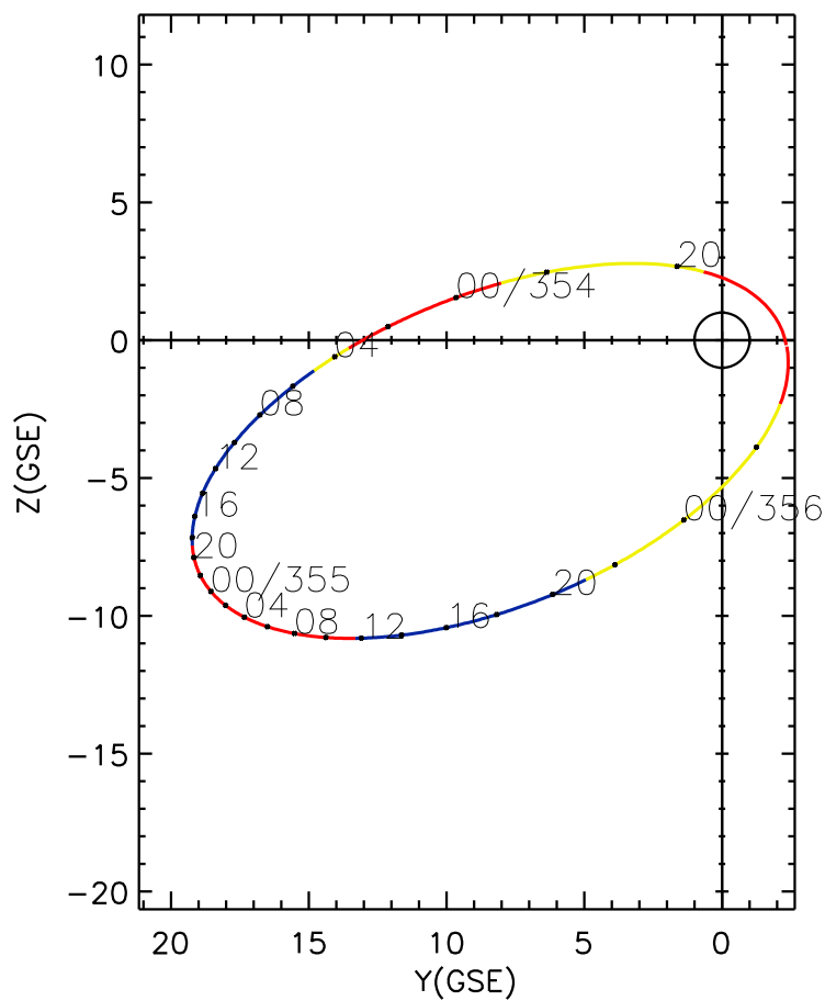
CLUSTER 2 orbit 2008 353 (12/18) 18:25 UT to 2008 356 (12/21) 03:31 UT
