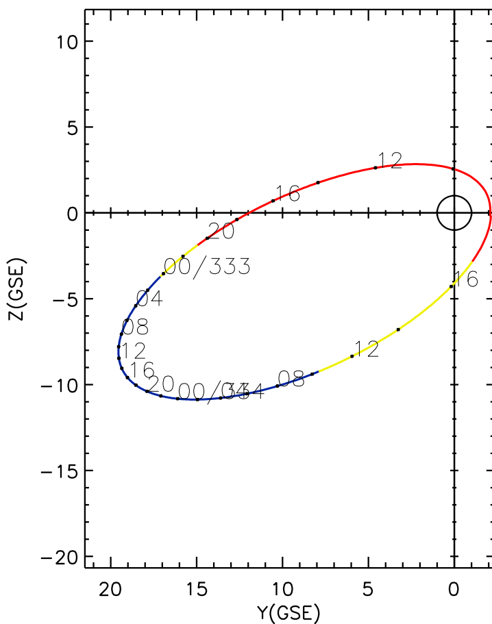
CLUSTER 2 orbit 2008 332 (11/27) 08:41 UT to 2008 334 (11/29) 17:46 UT
